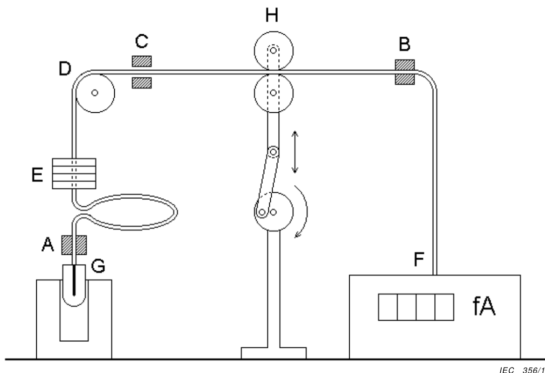
Figure B.1 – Test equipment for cable microphony
