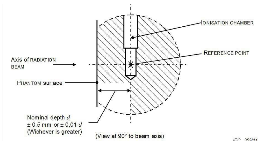
Figure 1 – Tolerance of depth in PHANTOM
